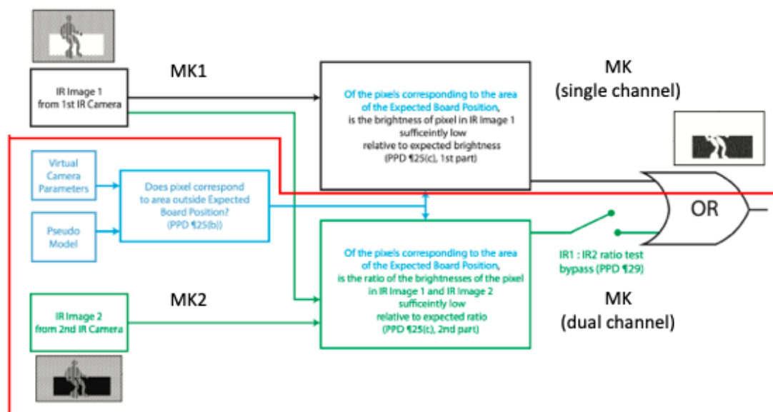
Figure how SVB System operates, provided by AIM Sport
